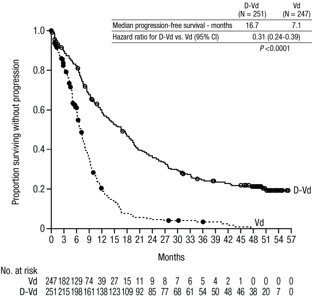
Figure 8: Kaplan-Meier curve of PFS in study MMY3004
