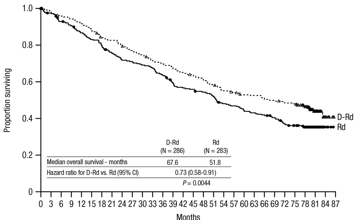
Figure 8: Kaplan-Meier curve of OS in study MMY3003
