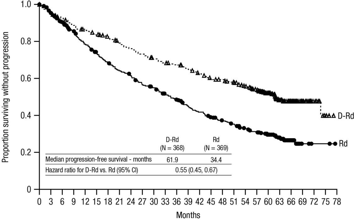
Figure 2: Kaplan-Meier curve of PFS in study MMY3008
