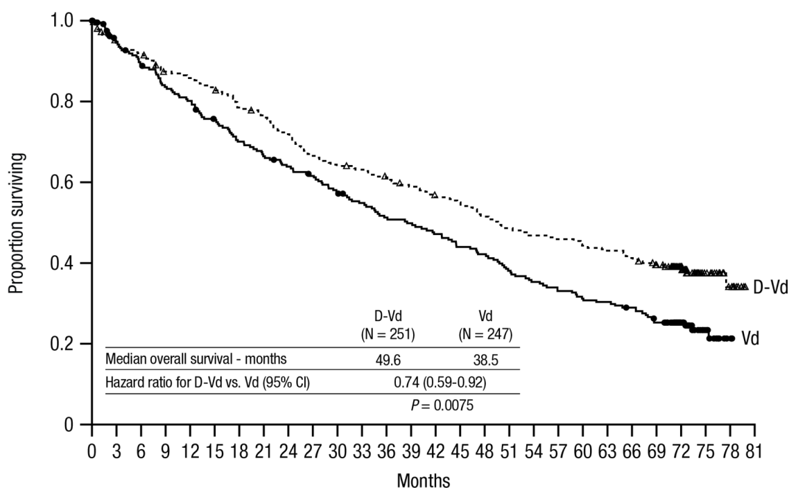
Figure 10: Kaplan-Meier curve of OS in study MMY3004
